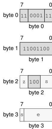
Figure 5-5. Long Encoding for ADC.X(z:B/W/L/Q) Rn(s), <ea>(e)
