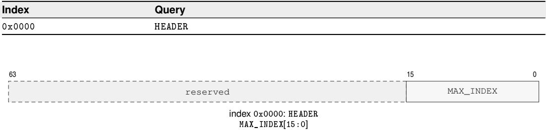
Figure 16-10. Control-Flow Integrity Discovery CPUID Result Formats
