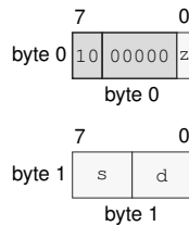
Figure 5-3. Short Encoding for MOV.X(z:L/Q) Rn(s), Rn(d)
