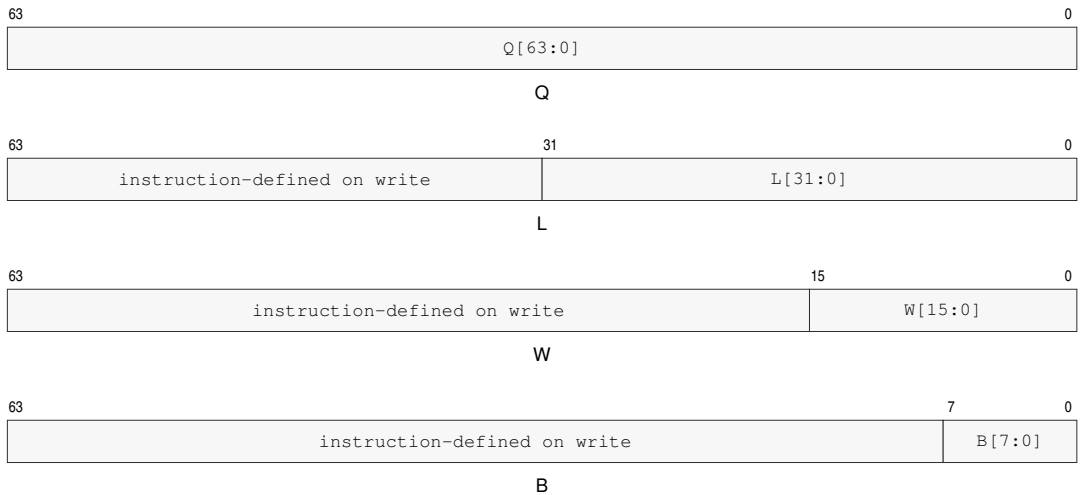
Figure 4-1. Rn Register Operand Subfields
