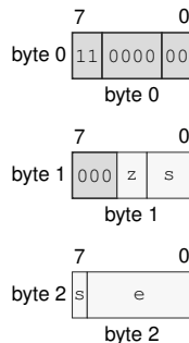
Figure 5-4. Medium Encoding for MOV.X(z:B/W/L/Q) Rn(s), <ea>(e)
