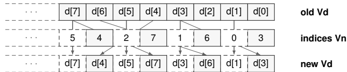
VPERM.W indexed lane selection
