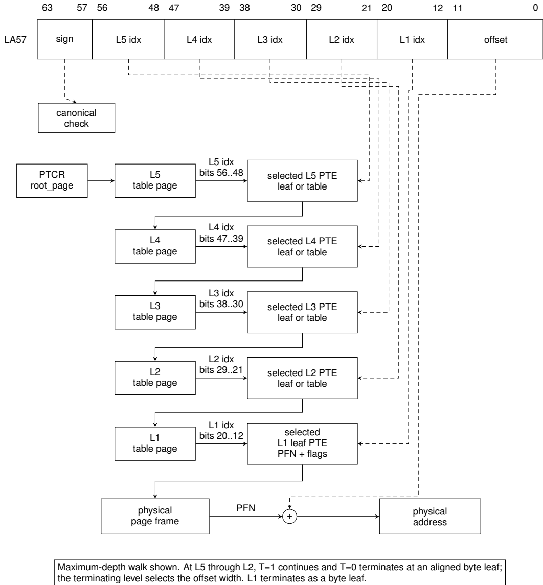
Figure 7-4. LA57 Five-Level Page Walk
