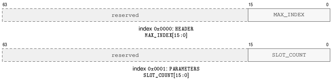
Figure 16-18. Architectural Debug Triggers CPUID Result Formats
