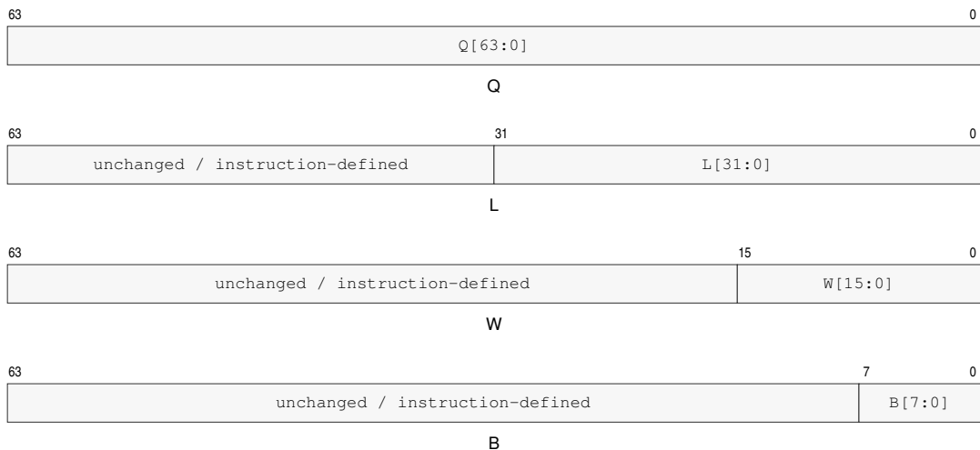
Figure 5-1. Integer Register Operand Subfields
