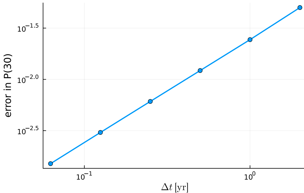
Figure 1: Error in P(30) against step size. The slope is the order of convergence.
