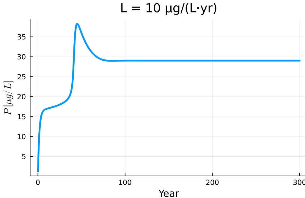
Figure 2: P(t) for the two-stock lake model at L = 10 \mu\text{g}/(\text{L}\cdot\text{yr}) .
