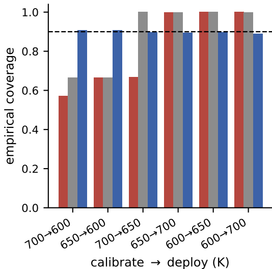
(a) catalyst testbed, \eta = 0
