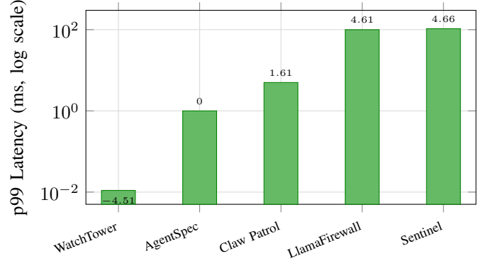
Fig. 4. p99 hot-path latency (log scale). WatchTower: 0.011 ms; AgentSpec: \sim 1 ms [4]; Claw Patrol: < 5 ms [5]; LlamaFirewall: > 100 ms [3]; Distributed Sentinel: 106 ms [6].
