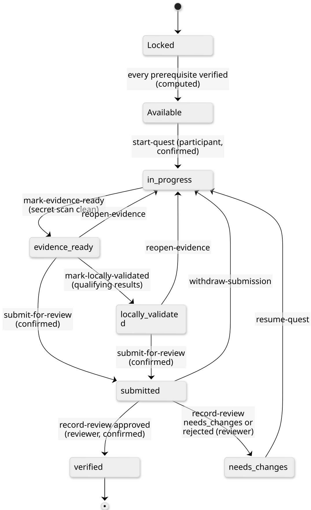
Figure 5. The attempt state machine as implemented in quest_app/state_machine.py (participant transitions) and quest_app/review.py (reviewer transitions). Locked and Available are computed in progress_calc.py and never written.
