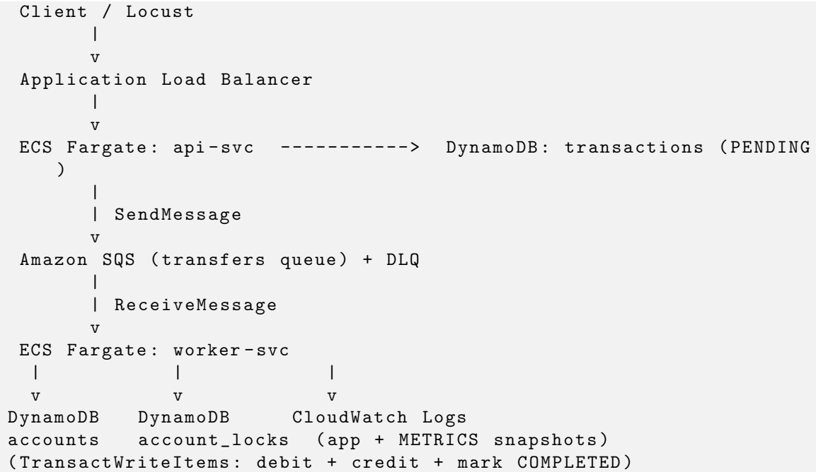
Figure 1: Deployed architecture. Every arrow crosses an AWS service boundary; no component runs locally.
