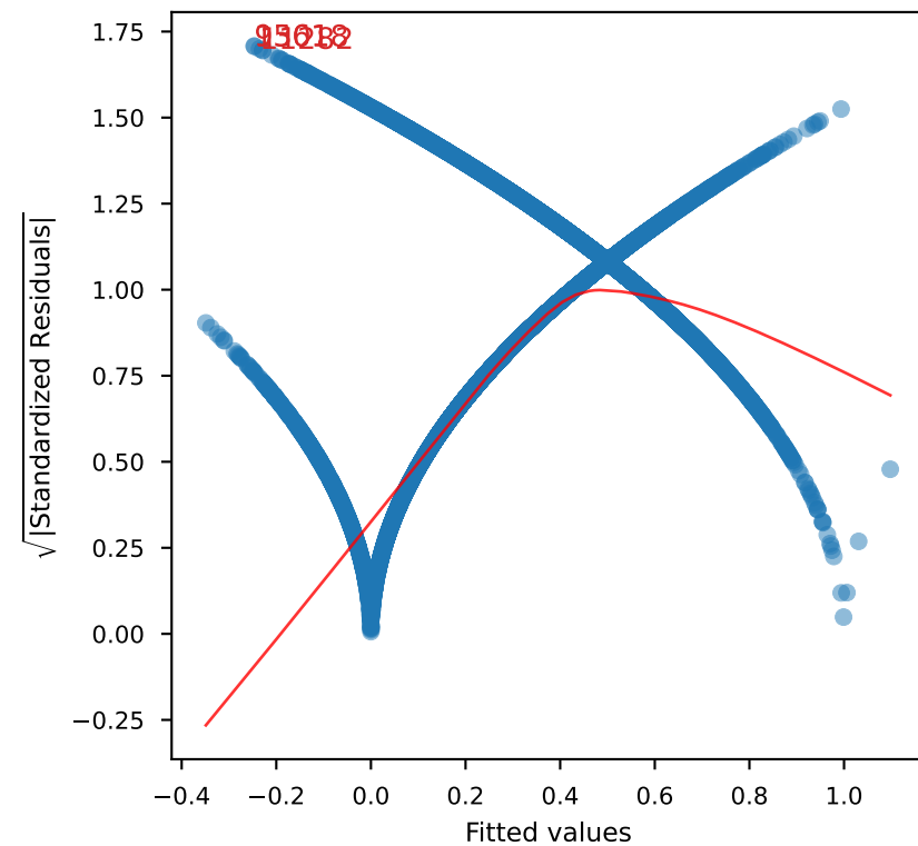
Scale-Location
