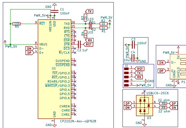
USB TO UART CONVERTER
