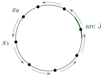
equal steps \theta < |J| : the walk laps the circle and cannot jump the arc
