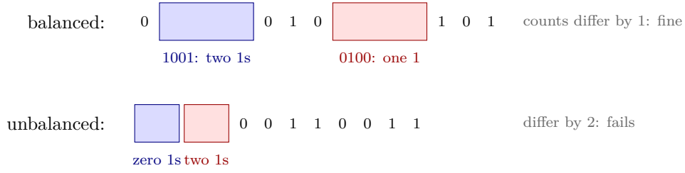
FIGURE 14. Balance, by sliding windows. Above, a balanced word: any two windows of the same length hold 1-counts differing by at most one, wherever you place them. Below, 00110011... fails at once — the windows 00 and 11 differ by two. Balance is the strongest possible “spread the 1s evenly” condition short of periodicity, and §13 shows it forces the word to track a straight line.
