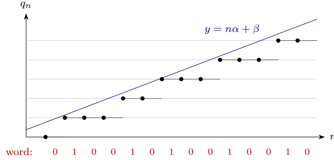
FIGURE 18. The second costume. The staircase q_n = \lfloor n\alpha + \beta \rfloor tracks the line, and the word beneath records where it steps (a 1) versus where it waits (a 0). Figure 6 showed the same object as a walk on the number line: a Beatty walk's gaps and a mechanical word's letters are two readings of one digitized line.
