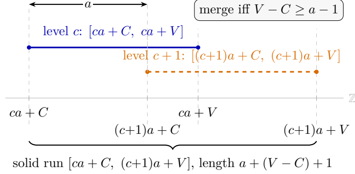
FIGURE 4. Two consecutive frames, offset by a , merge into one solid run of consecutive integers precisely when V - C \geq a - 1 .
