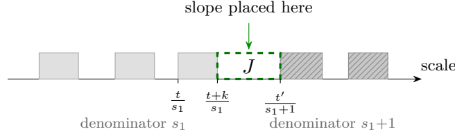
FIGURE 1. The unsafe intervals [t/s, (t+k)/s] that a lacunary B forces at denominators s_1 and s_1 + 1 , and the free gap J between them into which the construction places its slope. Ticks mark the endpoints t/s_1 and (t+k)/s_1 of the last denominator- s_1 interval and the start t'/(s_1+1) of the first denominator- (s_1+1) interval, where t' = t + k .
