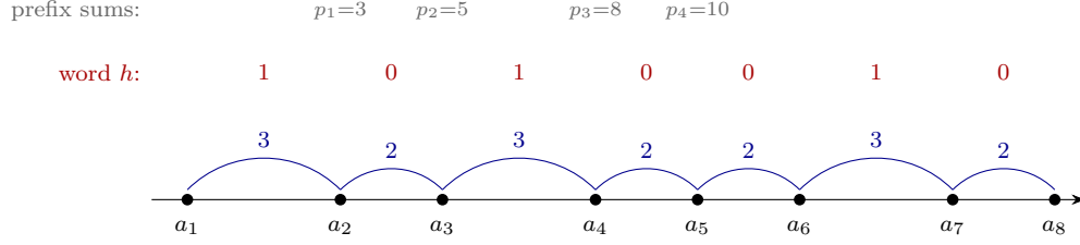
FIGURE 12. Four coordinate systems for one walk (gaps 3, 2, 3, 2, 2, 3, 2, ...; letters \delta = 2 , \delta' = 3 , so e = 1 ): the terms a_n on the line, the gaps g_n as arches, the binary word h (large step = 1), and the prefix sums p_n = a_{n+1} - a_1 . §§9–14 translate between these constantly; this figure is the dictionary.
