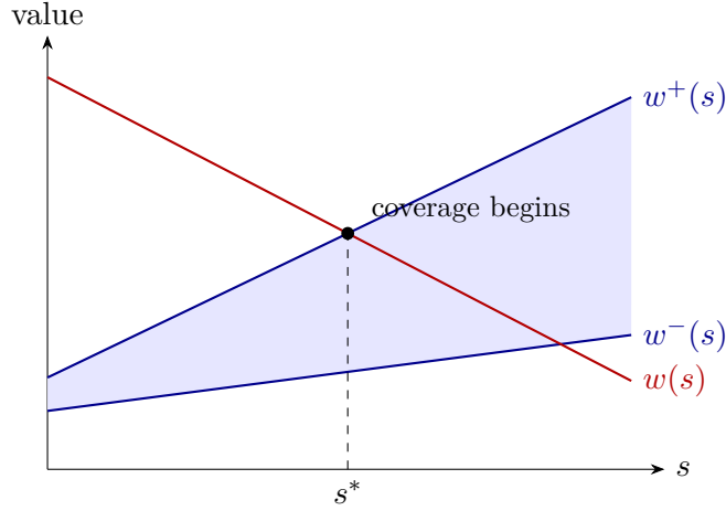
FIGURE 2. The window [w^-(s), w^+(s)] widens with s while the target w(s) descends into it; past the crossing s^* every large value is reachable.
