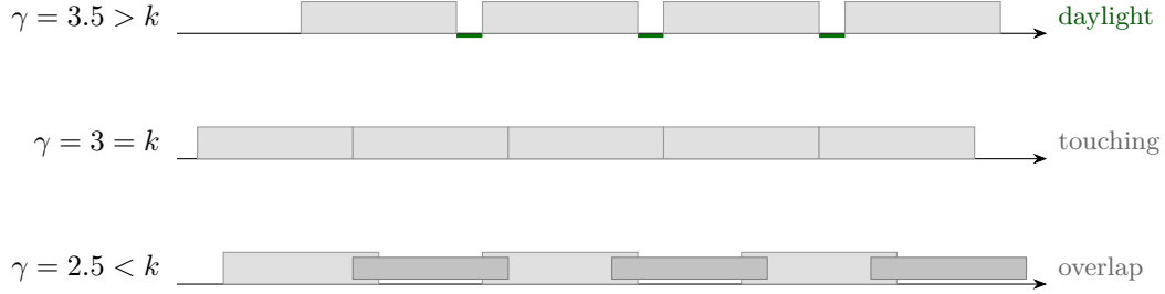
FIGURE 4. The dichotomy in one triptych ( k = 3 throughout): windows of width 3 at stride \gamma . Above the threshold ( \gamma > k ) daylight recurs forever; at \gamma = k the windows tile the line exactly; below ( \gamma < k ) they overlap. The theorem says the picture tells the truth: the game is winnable precisely when a stride \gamma > k is available, i.e. when d_2 \geq k + 1 . (One caution the proof will respect: daylight makes dodging possible , never automatic — integer strides above k still lose. See the closing remark of §6.)
