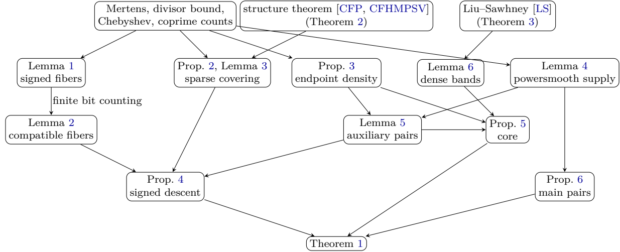
Figure 2: Dependencies among the main statements.
