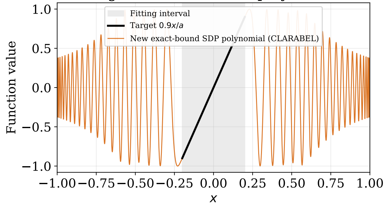
Degree 101: new SDP polynomial
