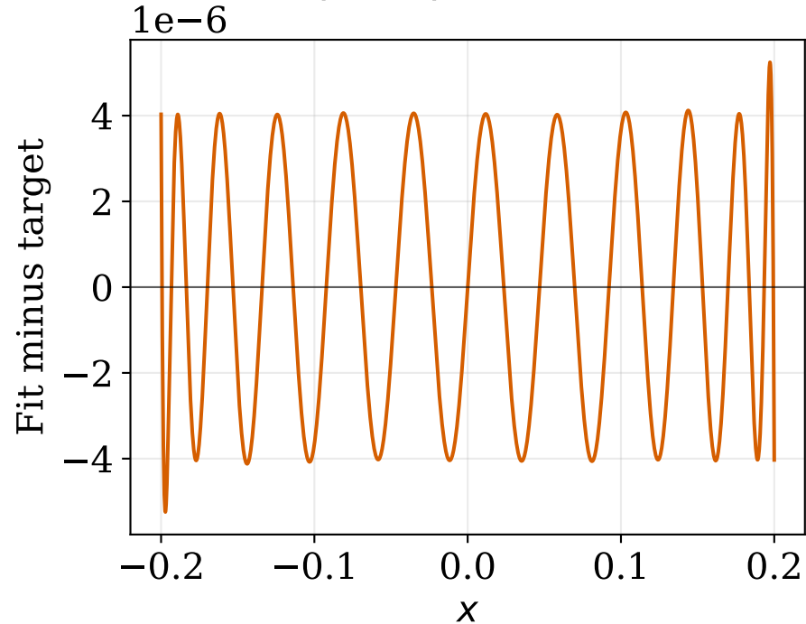
Pointwise error \max |p - f| = 5.25e - 06
