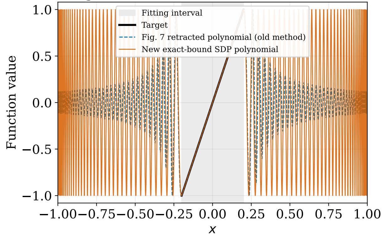
Degree 181: old retraction vs new SDP
