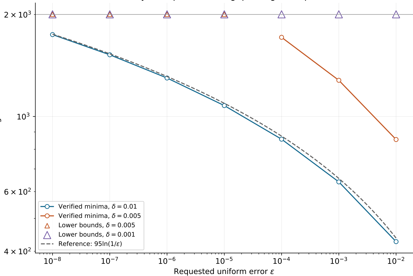
Accuracy sweep at smaller gaps (degree cap: 2001)
