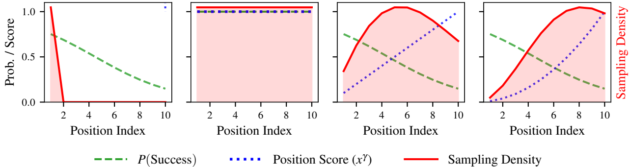
(a) Root Only ( \gamma \ll 0 )
