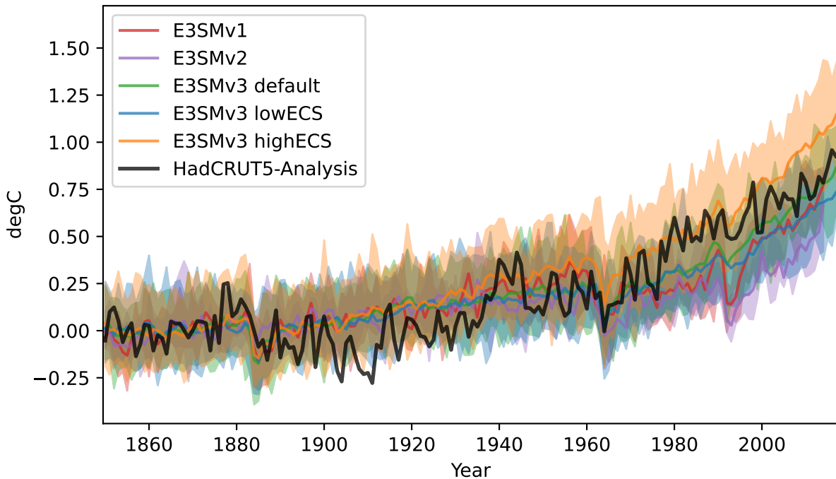
SH surface temperature anomaly (ref 1850-1899)
