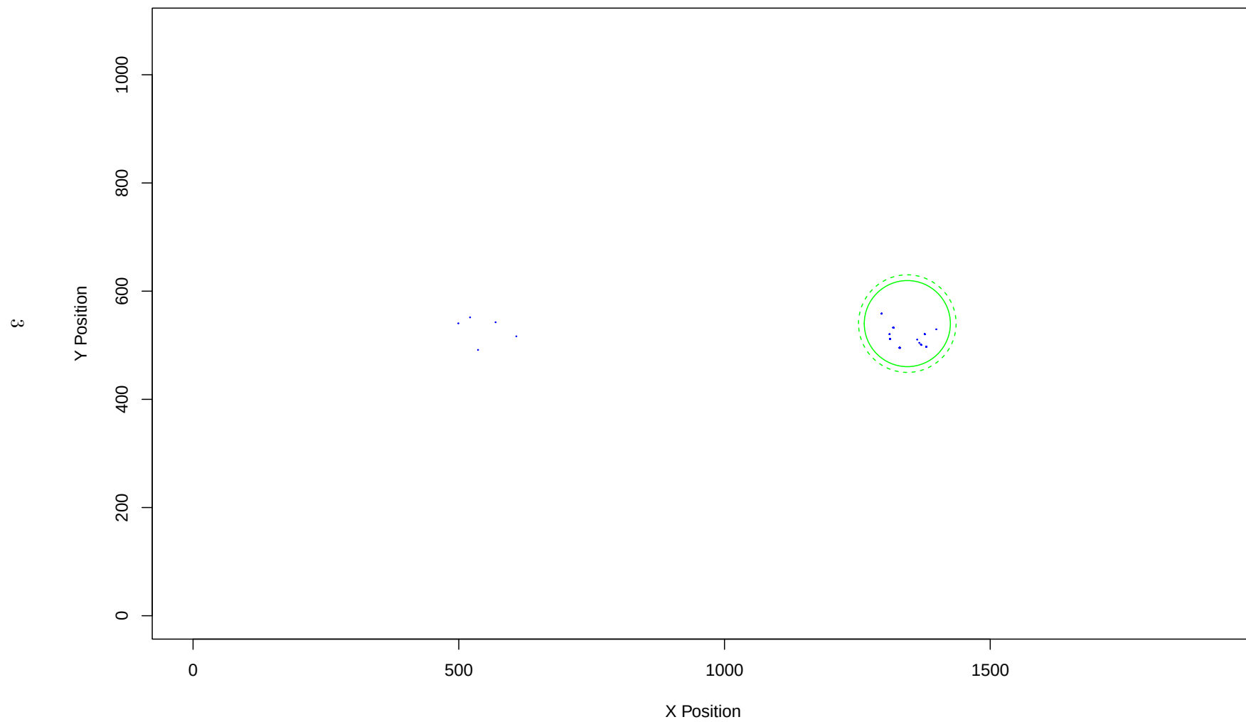
Pecks Distribution
