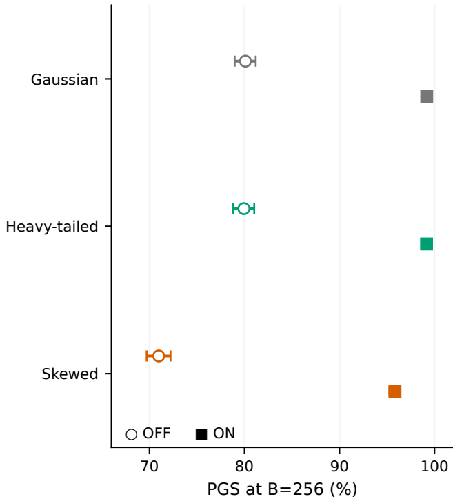
b Known-mean stress, M=5,000
