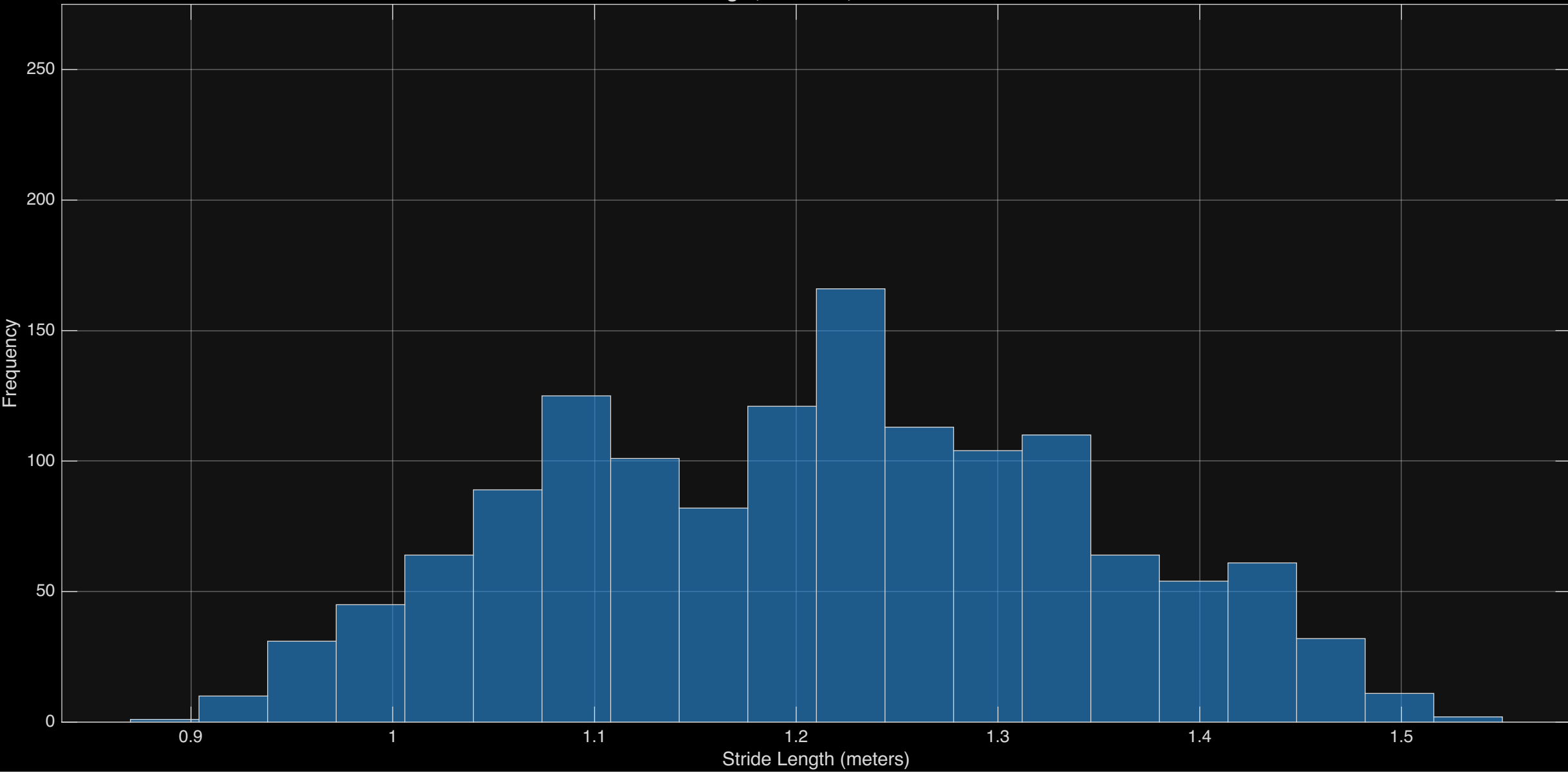
Stride Length, Incline i5, No acceleration
