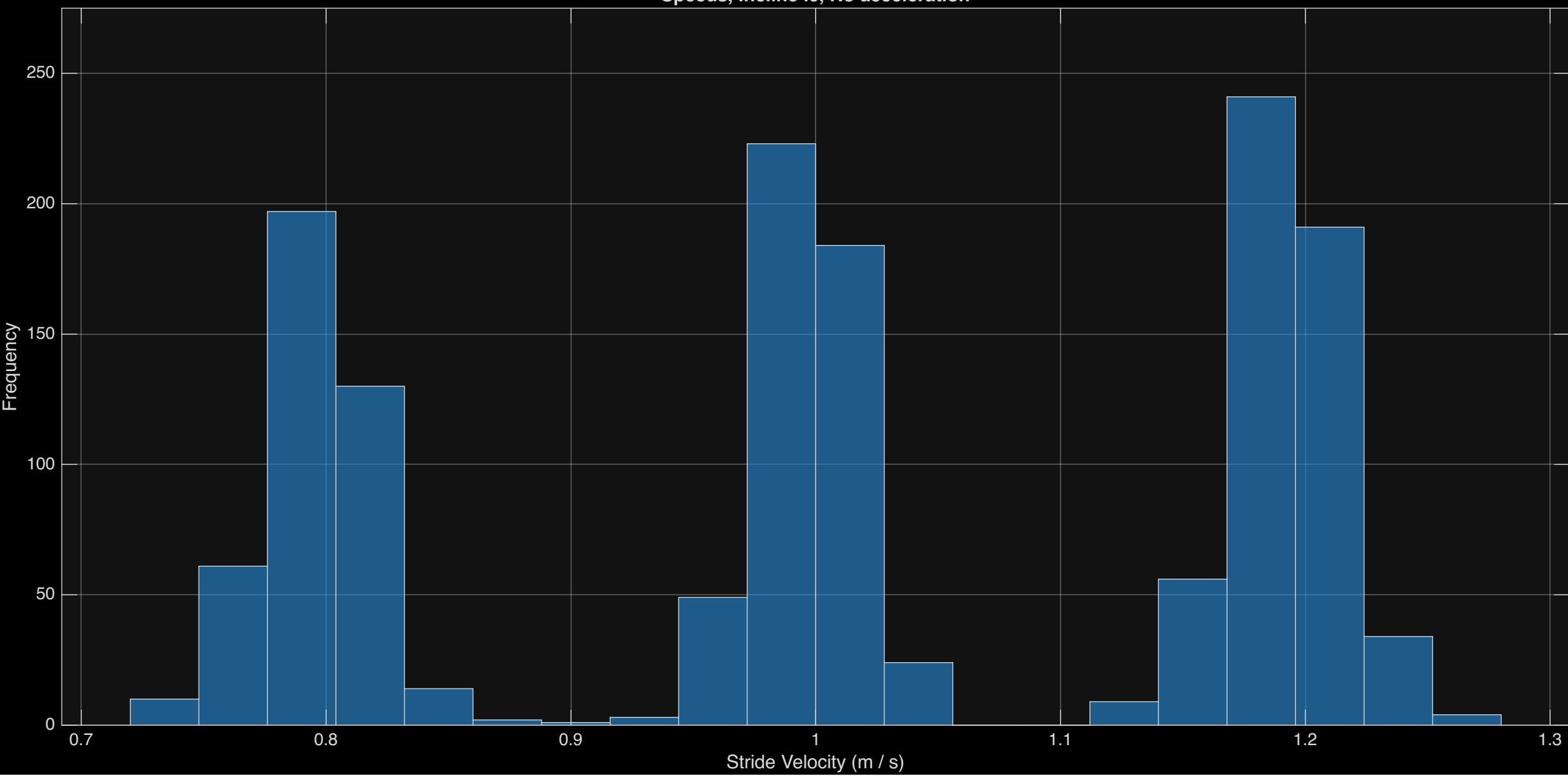
Speeds, Incline i0, No acceleration
