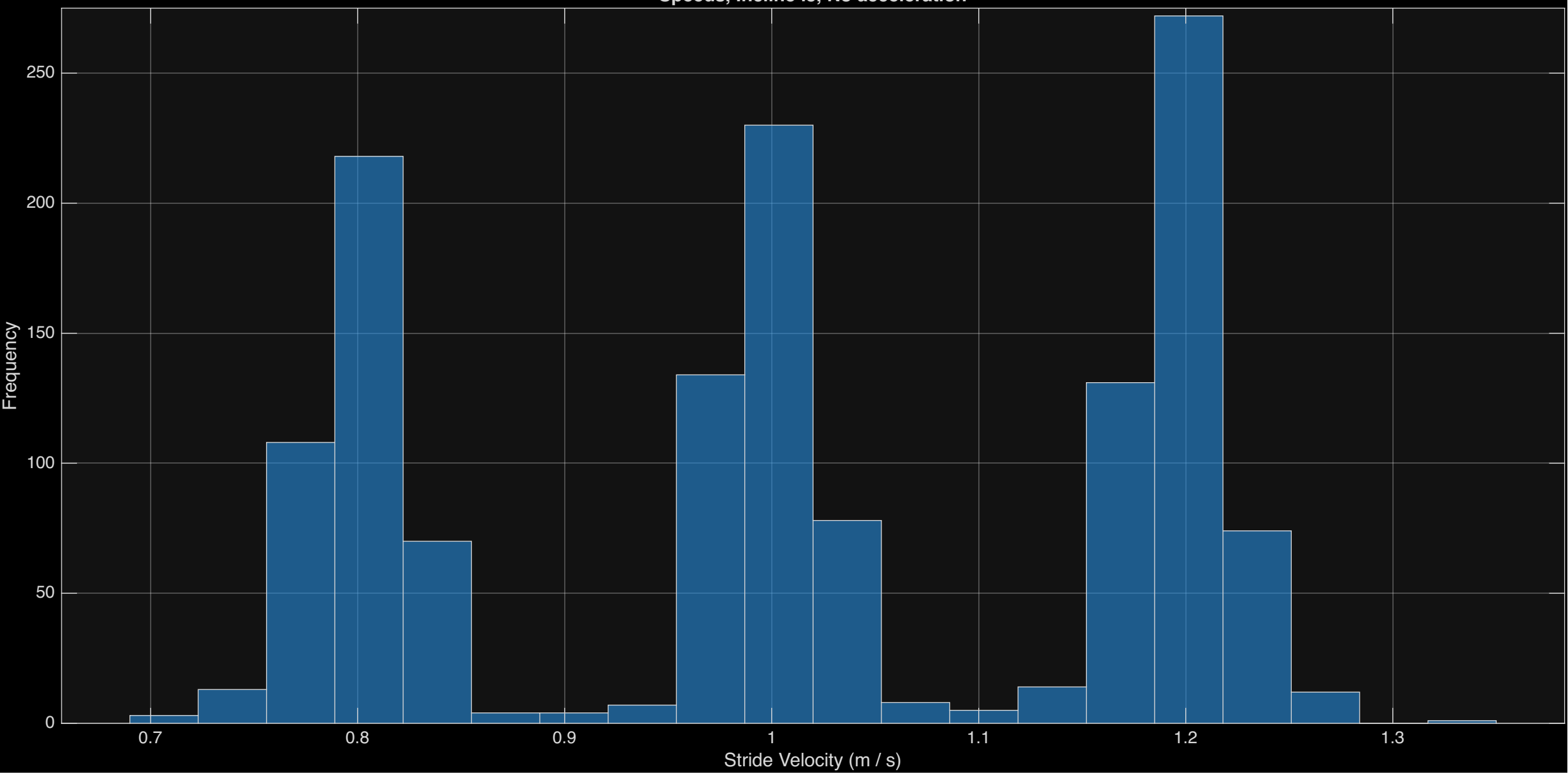
Speeds, Incline i5, No acceleration
