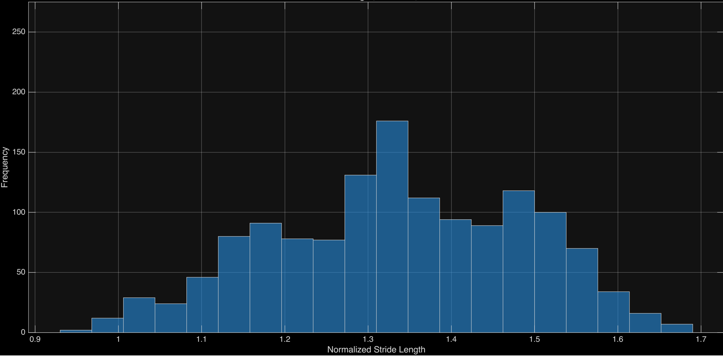
Normalized Stride Length, Incline i5, No acceleration
