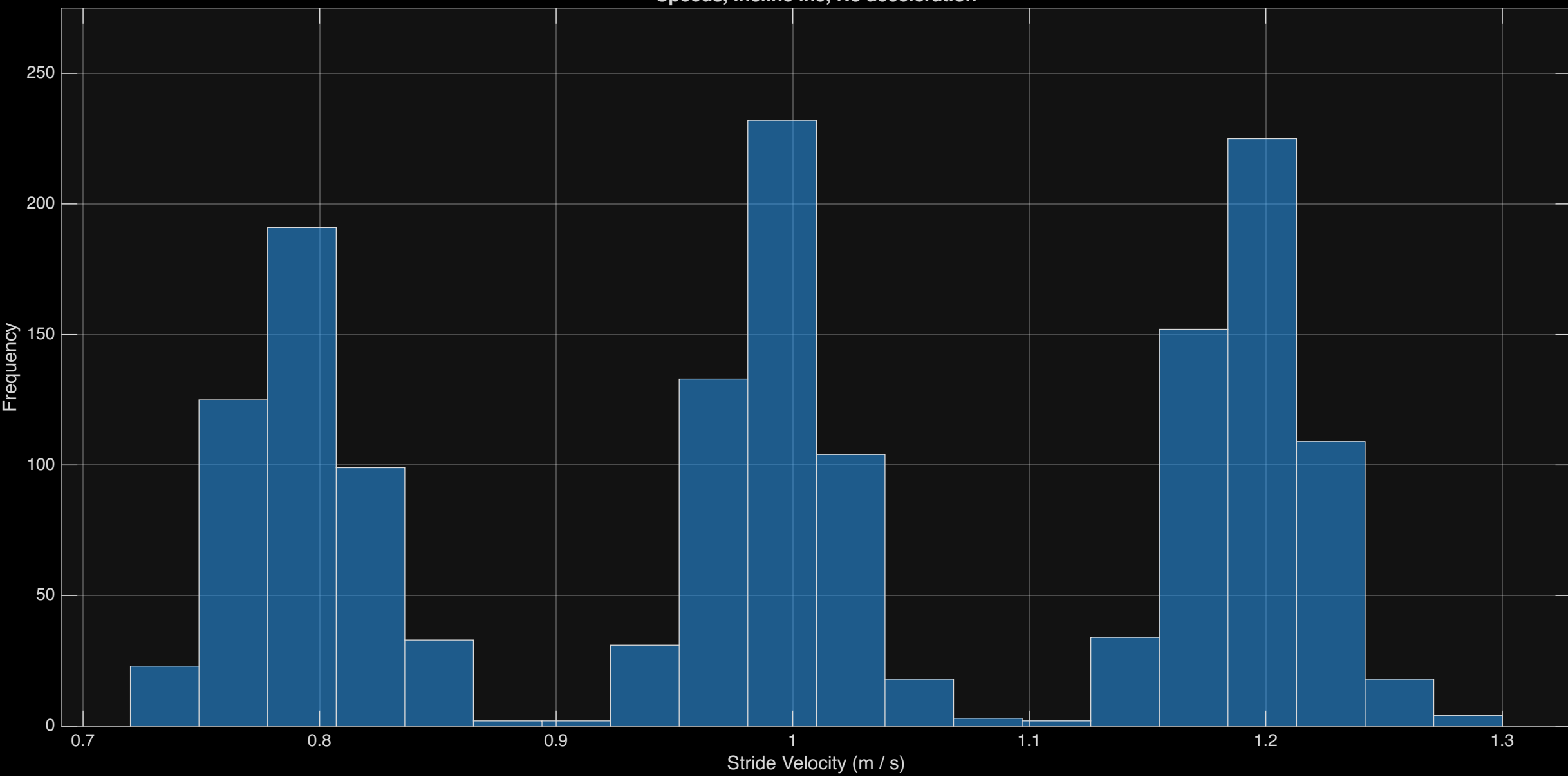
Speeds, Incline in5, No acceleration
