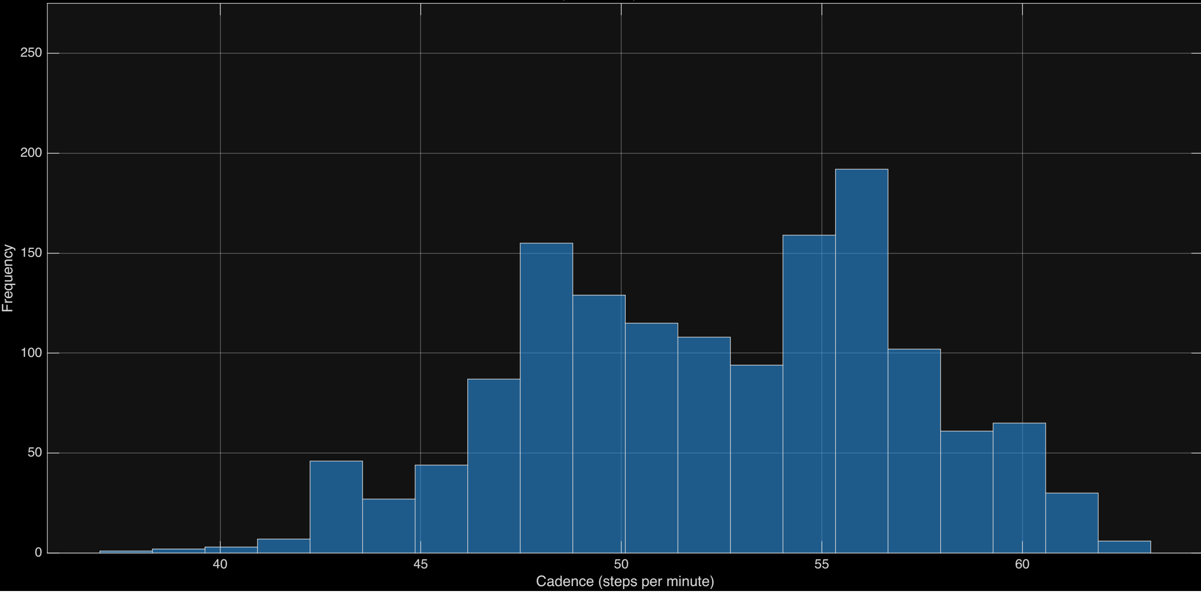
Cadence, Incline i0, No acceleration
