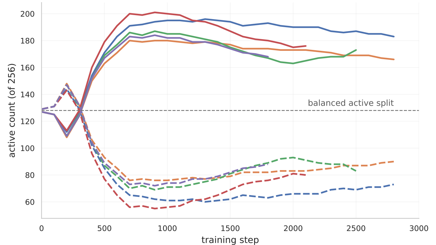
Routing specialization diagnostics
