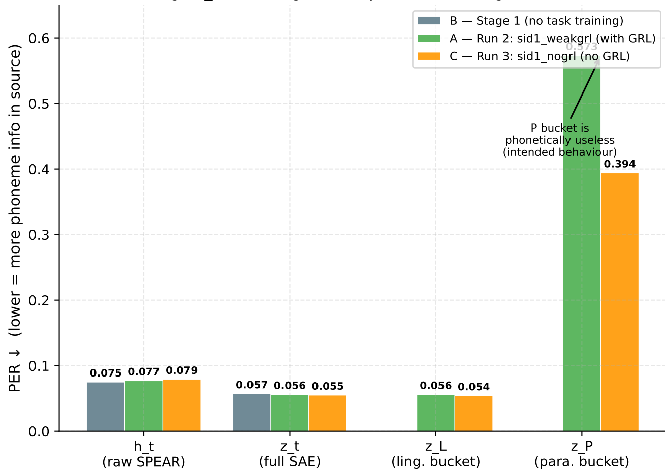
PR Phoneme Error Rate by Source High z_P \rightarrow \text{PER} = good (no phoneme leakage into P)
