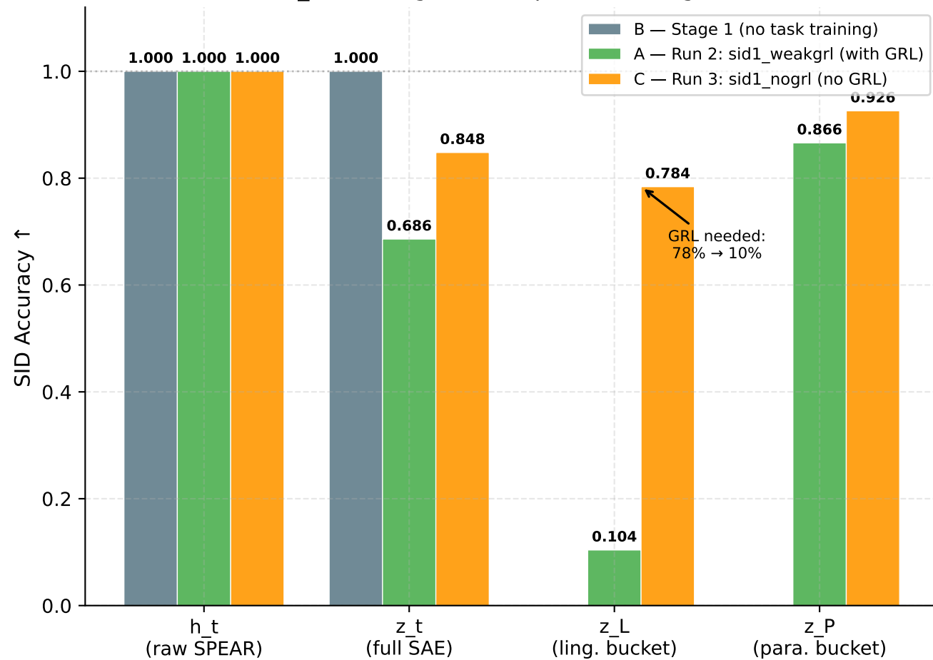
SID (Speaker ID) Accuracy by Source Low z_L \rightarrow \text{SID} = good (no speaker leakage into L)
