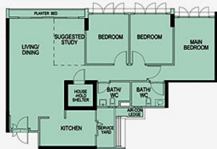
TYPICAL 5-ROOM FLOOR PLAN APPROX. FLOOR AREA 115 sqm (Inclusive of Internal Floor Area 110 sqm, Air-Con Ledge and Planter Bed)
