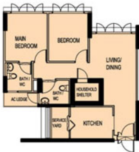
TYPICAL 3-ROOM FLOOR PLAN APPROX. FLOOR AREA 68 sqm (Inclusive of Internal Floor Area 65 sqm and Air-Con Ledge)
