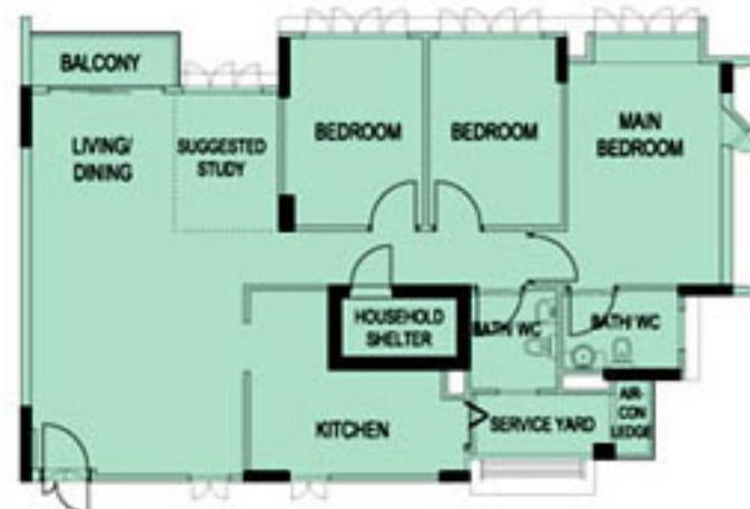
TYPICAL 5-ROOM FLOOR PLAN APPROX. FLOOR AREA 116 sqm (Inclusive of Internal Floor Area 114 sqm, Air-Con Ledge and Bay Window)
