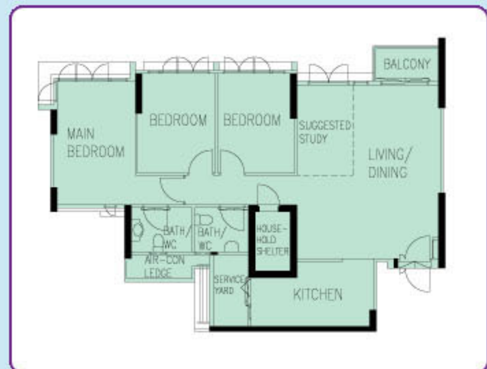
TYPICAL 5-ROOM FLOOR PLAN WITH BALCONY APPROX. FLOOR AREA 113 sqm (Inclusive of Internal Floor Area 110 sqm and Air-Con Ledge)
