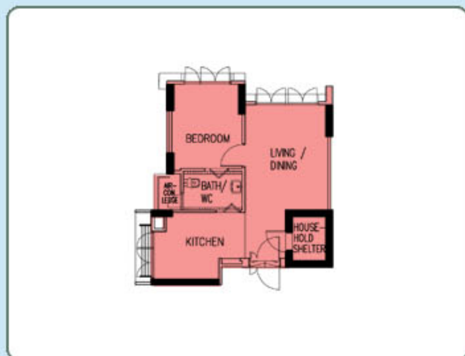
TYPICAL 2-ROOM FLOOR PLAN APPROX. FLOOR AREA 44 sqm (Inclusive of Internal Floor Area 42 sqm and Air-Con Ledge)
