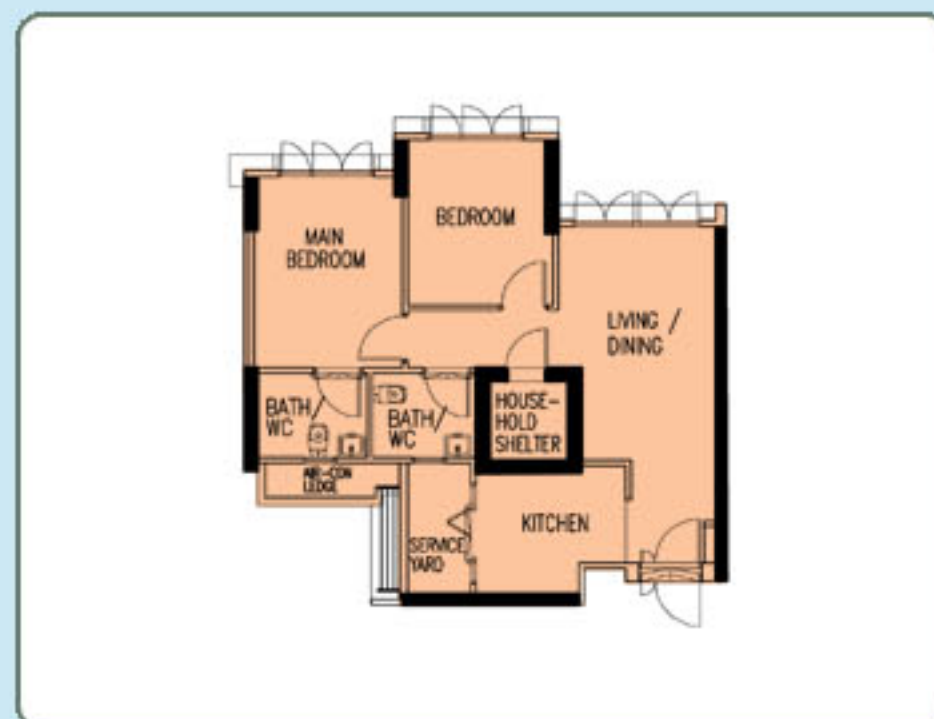
TYPICAL 3-ROOM FLOOR PLAN APPROX. FLOOR AREA 65 sqm (Inclusive of Internal Floor Area 62 sqm and Air-Con Ledge)
