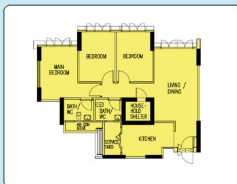
TYPICAL 4-ROOM FLOOR PLAN APPROX. FLOOR AREA 90 sqm (Inclusive of Internal Floor Area 87 sqm and Air-Con Ledge)
