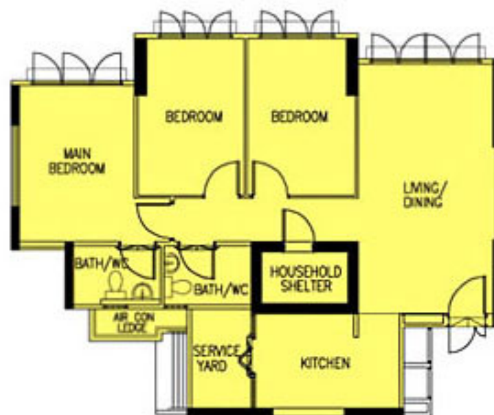
TYPICAL 4-ROOM FLOOR PLAN
