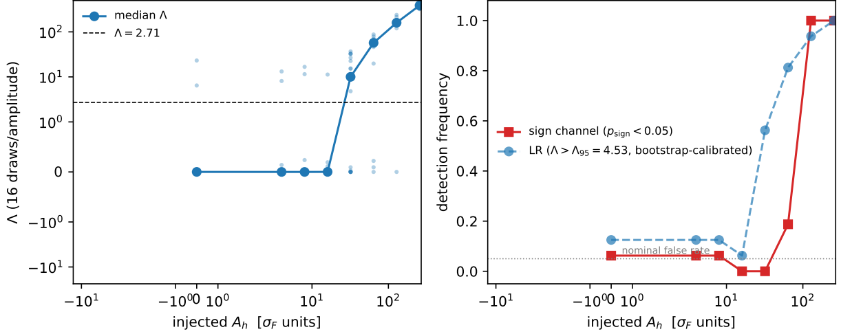
Figure 4: Injection recovery on real-data-conditioned resamples (v0.3.1 pipeline, 64 s / 64 log bins, 16 draws per amplitude). Left: \Lambda versus injected amplitude in units of the naive Fisher scale \sigma_F ; the likelihood ratio turns on near 30\sigma_F (v0.3, with its stalled optimizer, reported zeros across this entire axis). Right: detection frequency of both channels — the corrected LR and the fit-free sign-channel statistic ( p_{\text{sign}} < 0.05 ).
