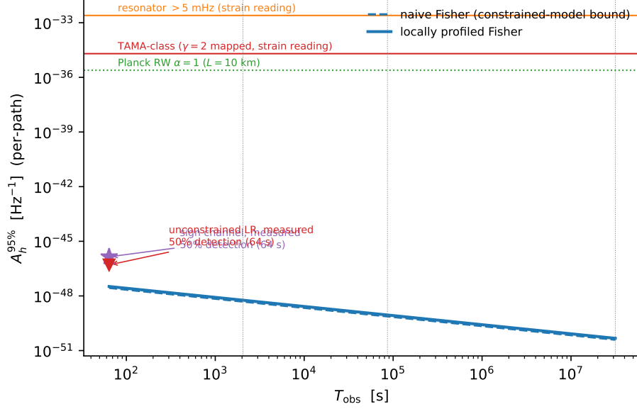
Figure 6: Projected ET sensitivity to S_h(f) = A_h(f/f_0)^{-2} (per-path): naive Fisher (dashed) and profiled Fisher (solid band edge) against existing bounds. All curves are path-template forecasts ( \mathbf{R} = \mathbf{I} ); under the strain reading, for which the bounds comparison shown is the favorable one, the forecast is provisional pending full-response injections (Section 10.2). Under the path-length reading the comparison changes qualitatively.
