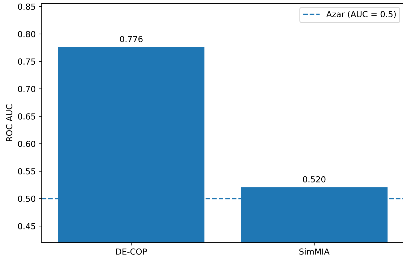
DE-COP vs. SimMIA — BookTection medium Llama-3.3-70B-Versatile
