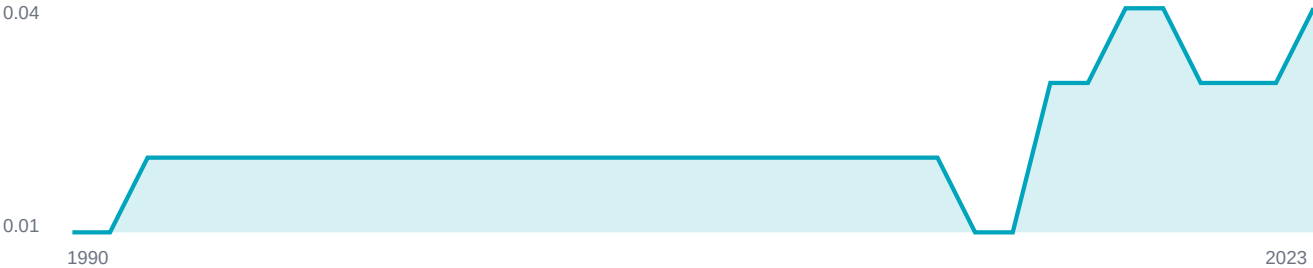
Transport CO2 emissions (Mt), 1990–2023, EDGAR
