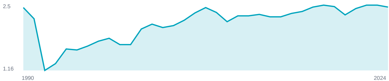
Transport CO 2 emissions (Mt), 1990–2024, EDGAR
