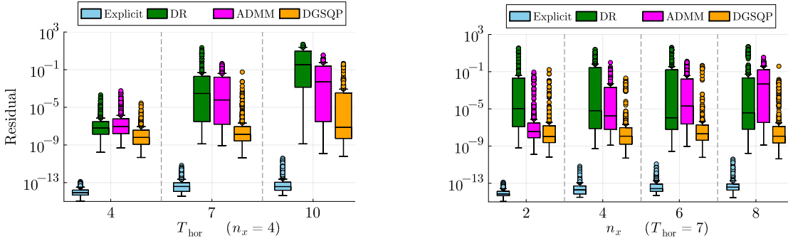
Fig. 4: Solution quality, measured by the natural residual [8, § 6], of the explicit mapping computed with Alg. 1, compared with that obtained by the DR [34], ADMM [26], and DGSQP [?] solvers under a computational budget of 0.1 s. The left plot reports the results as a function of the horizon length, and the right plot as a function of the state dimension.
