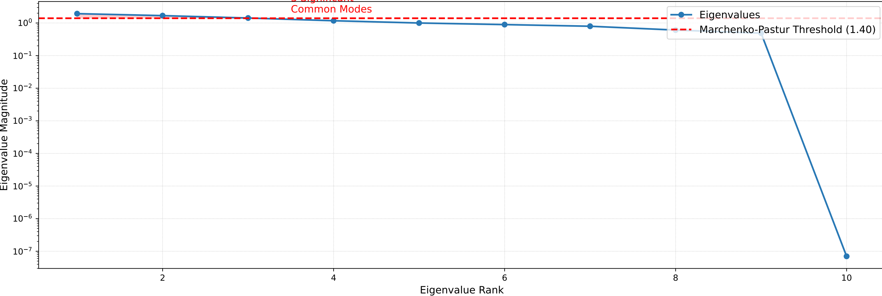
Phase 2: RMT Eigenvalue Spectrum (Common vs Idiosyncratic Shocks)
