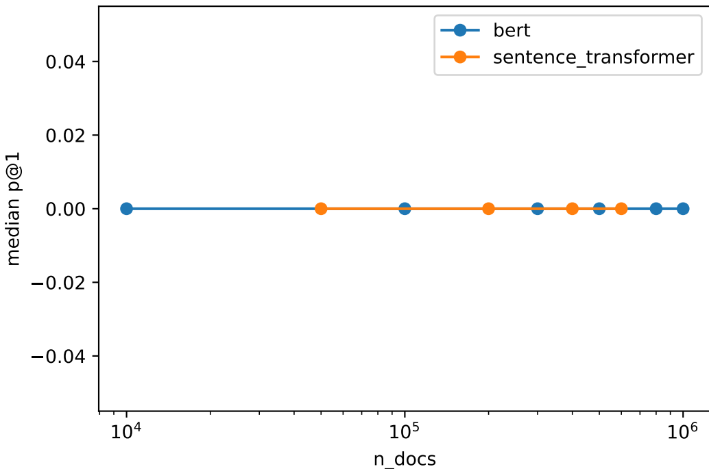
H3: model p@1 vs corpus size
