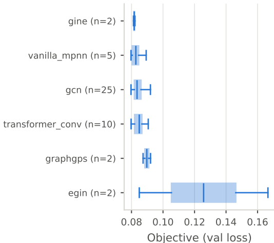
Objective by encoder
