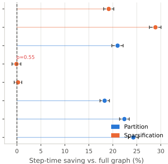
Step-time saving
