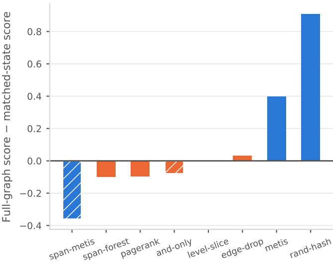
Cost of the structural shift (positive = the model does BETTER on full graphs)
