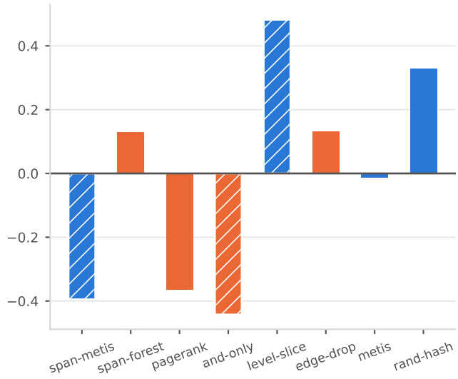
Cost of the structural shift (positive = the model does BETTER on full graphs)
