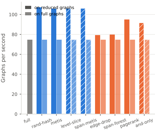
Inference throughput
