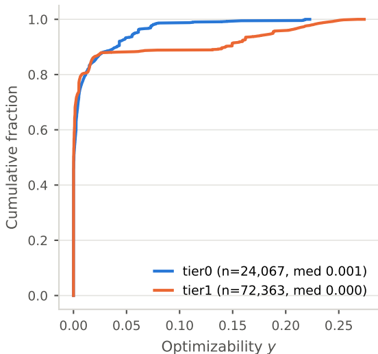
Label distribution by tier
