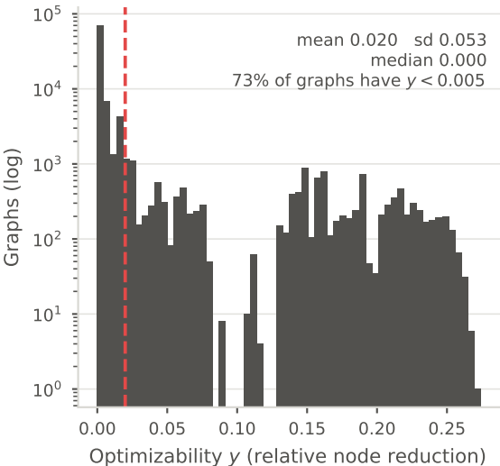
Pooled label distribution
