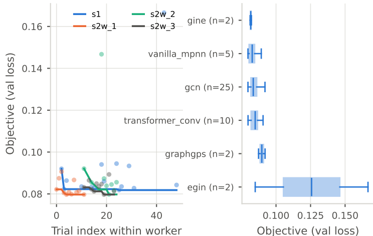
Sweep progress (6 outliers clipped) Objective by encoder
