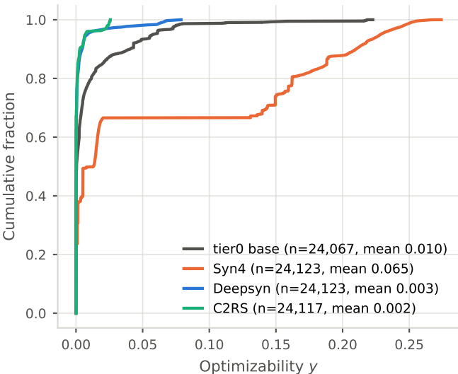
Label distribution by source script
