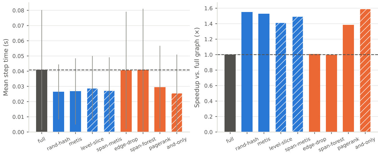
Training throughput across reduction methods (error bars: \pm 1 s.d. of step time over graphs) Training step time (dashed: full-graph baseline) Speedup under-delivers relative to compression
