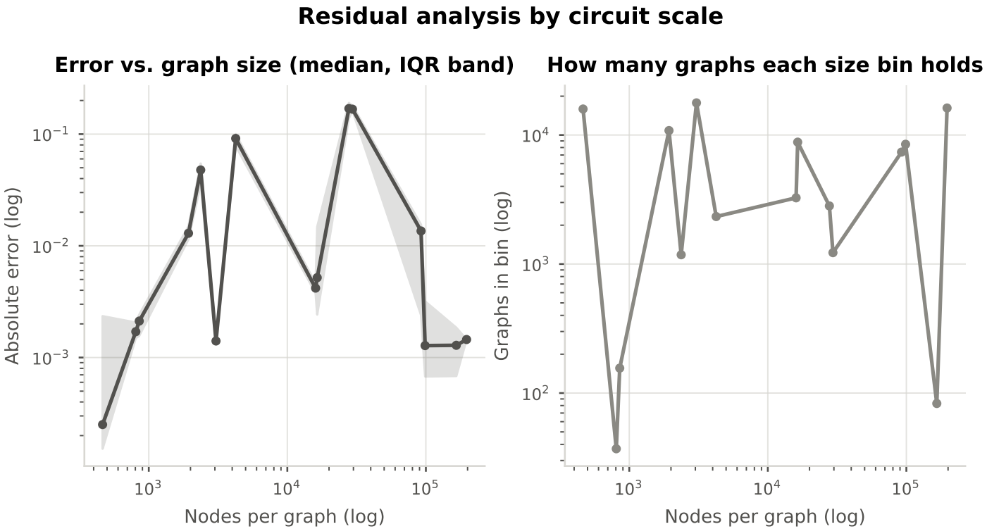
Figure 4.7: Absolute error of the full-graph baseline against graph size (median and interquartile band), with the number of graphs per size bin alongside so that a wide band on a thin bin is not read as a trend.
