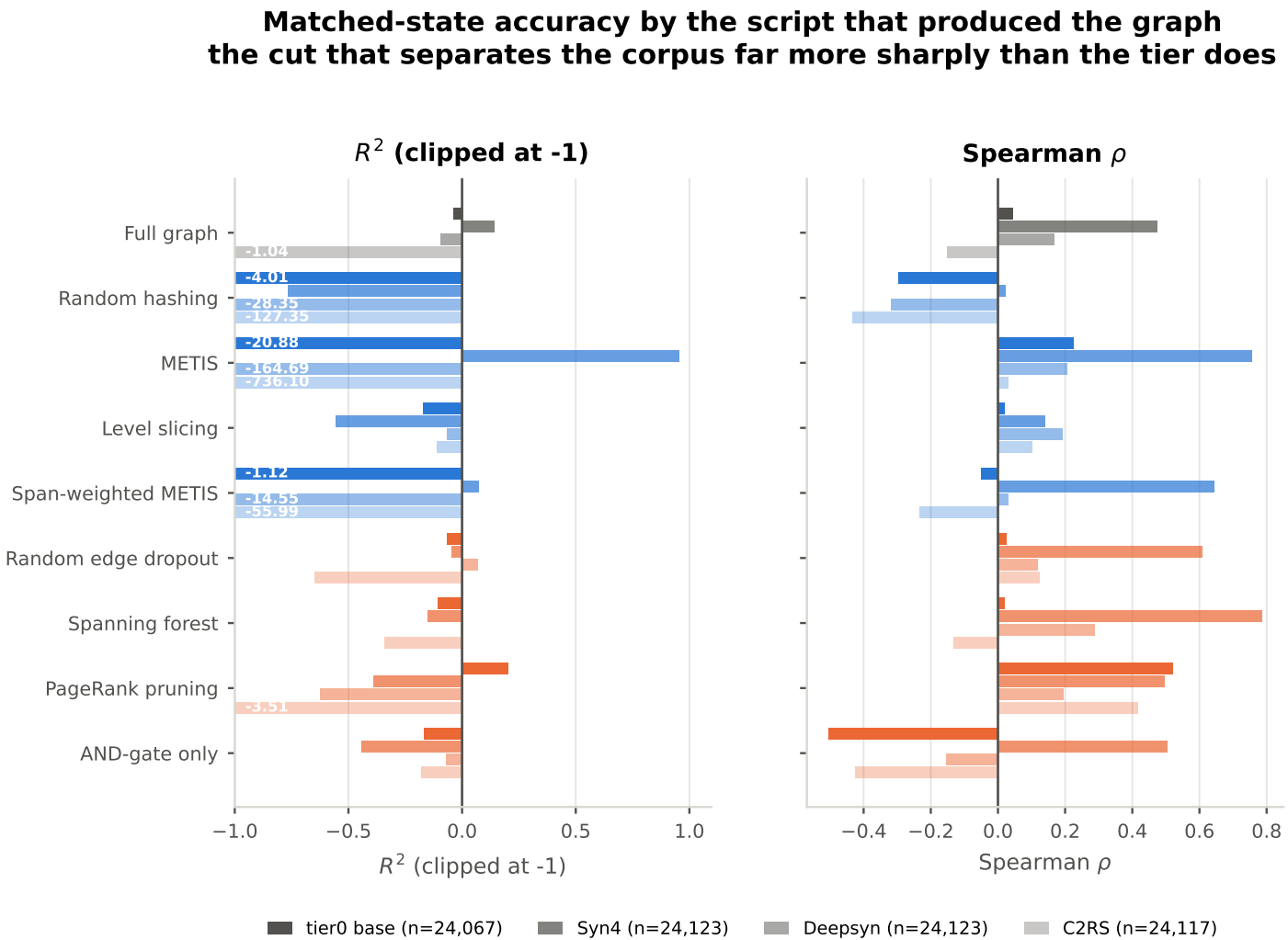
Figure 4.28: The same partition taken by the synthesis script that produced each graph, which separates the corpus far more sharply than the tier does (4.5). Every configuration degrades from Syn4-derived graphs to C2RS-derived ones.
